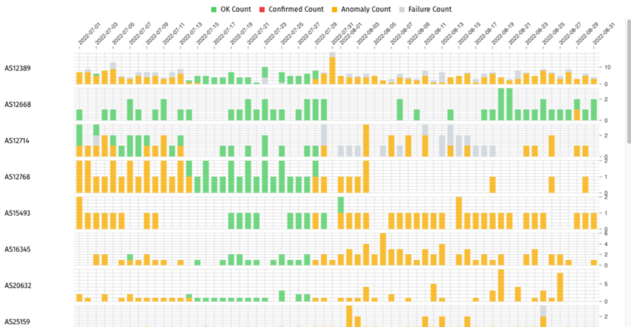
Chart: Per-ASN breakdown of OONI Probe testing coverage of www.torproject.org in Russia between 1st July 2022 to 1st September 2022 (source: OOONI data ).
