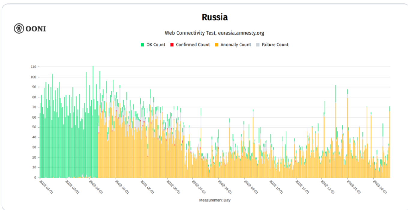
Chart: OONI Probe testing of eurasia.amnesty.org on 418 ASNs in Russia between 1st January 2022 to 20th February 2023 (source: OONI data ).
