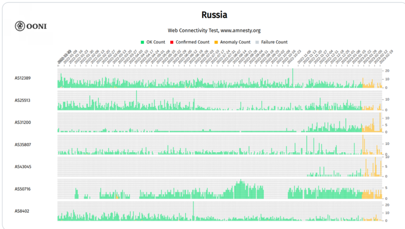
Chart: ASNs in Russia which presented the largest volume of anomalies (more than 50) in the testing of www.amnesty.org between 1st January 2022 to 21st February 2023 (source: OONI data ).
