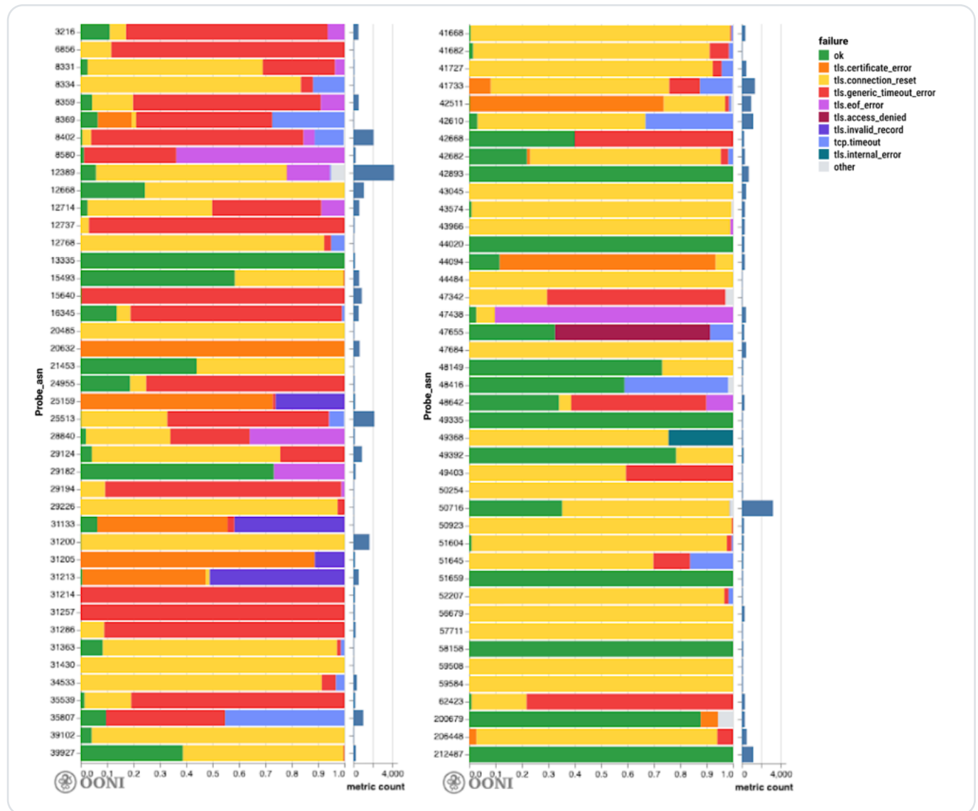
Chart: Measurement failures observed when www.patreon.com was tested on different ASNs in Russia between 6th August 2022 to 18th February 2023 (source: OONI data).
