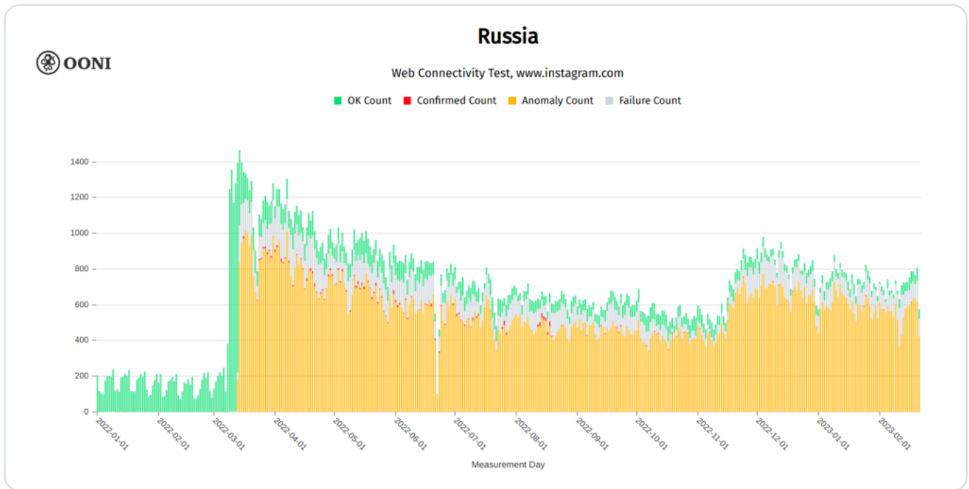
Chart: OONI Probe testing of Instagram ( www.instagram.com ) on 797 ASNs in Russia between 1st January 2022 to 21st February 2023 (source: OONI data ).
